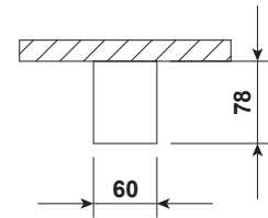
Standard surface mounted version
